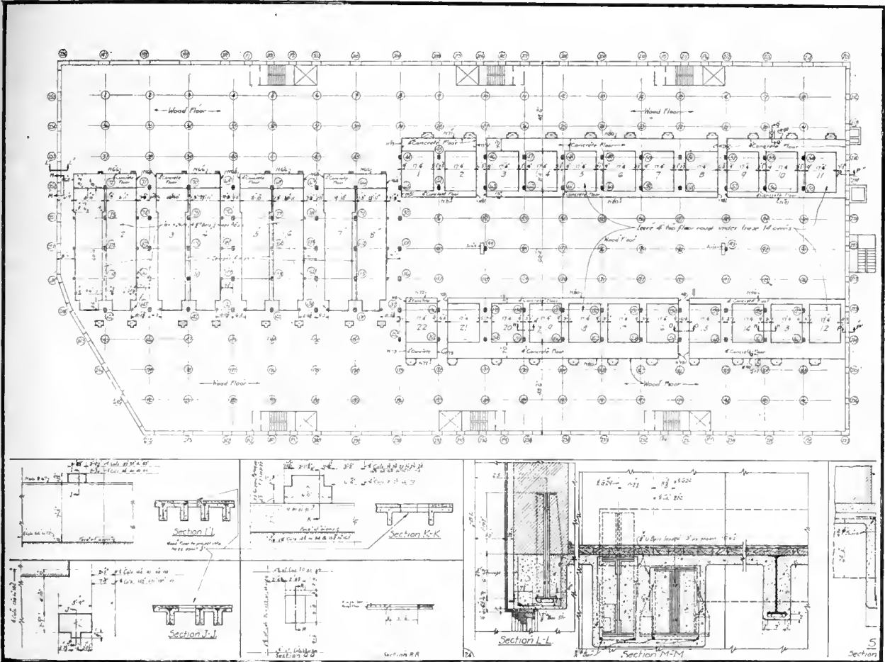
PLAN OF SEVENTH FLOOR Showing location of English and American bake ovens
